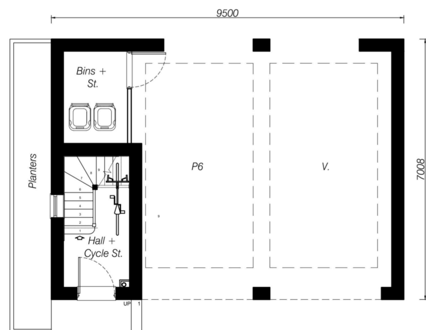
Ground Floor Plot 6 1b2p 56m2 total GIA
