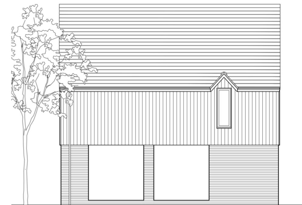
Rear Elevation
