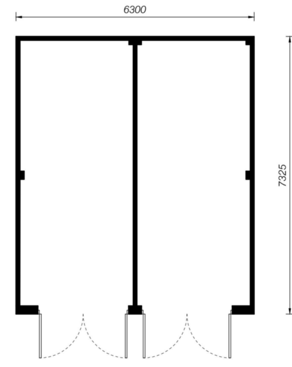
G1/2 Garage Floor Plan
